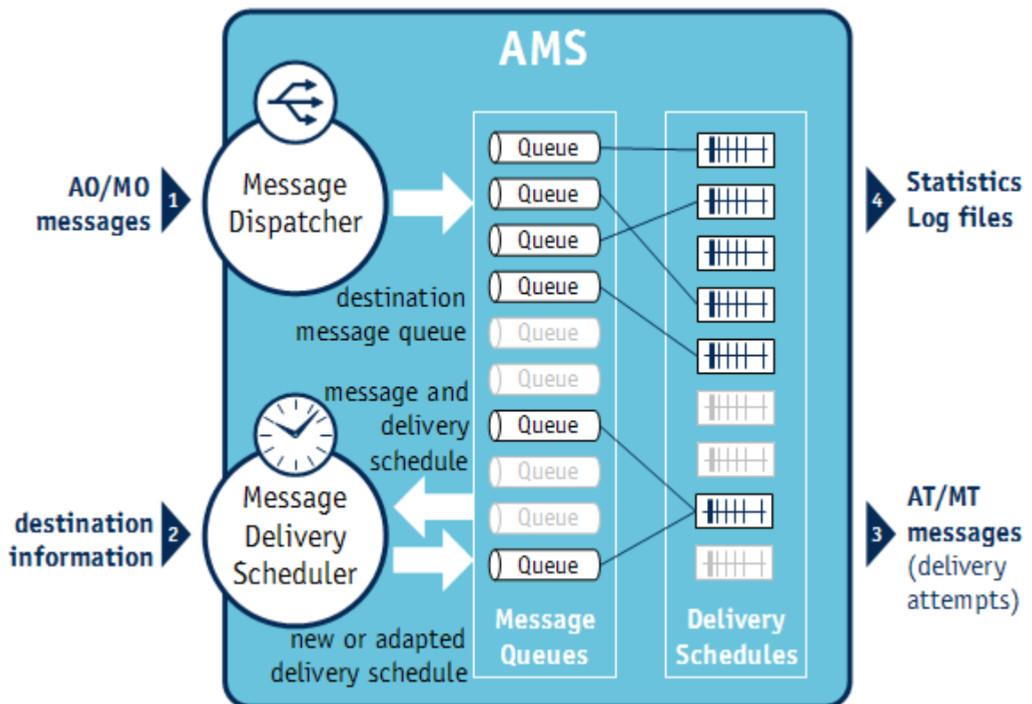
Figure 3: Message dispatcher and delivery scheduler
